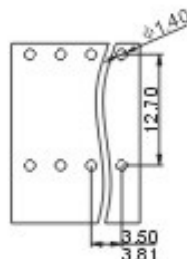
PCB LAYOUT
