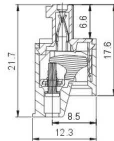
Section B-B
