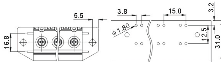
PCB LAYOUT
