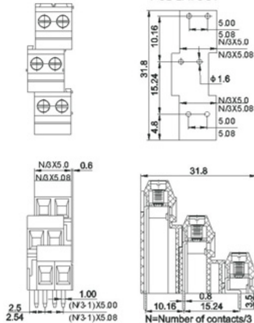
PCB LAYOUT
